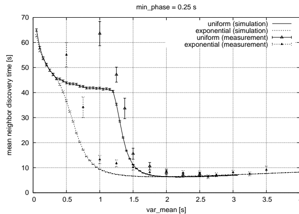
Figure 3: Mean neighbor discovery time: Simulation and measurement results for uniform and exponential distribution of var_phase.
