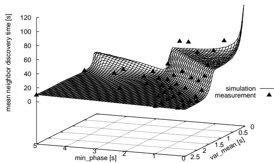
Figure 2: Mean neighbor discovery time: Simulation and measurement results.
